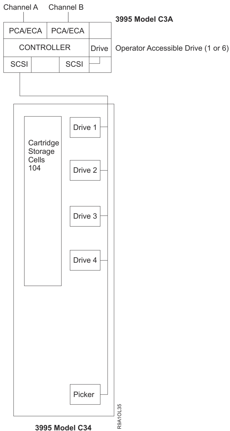
Figure 35. Sample Hardware Configuration—IBM 3995 Models C3A and C34
