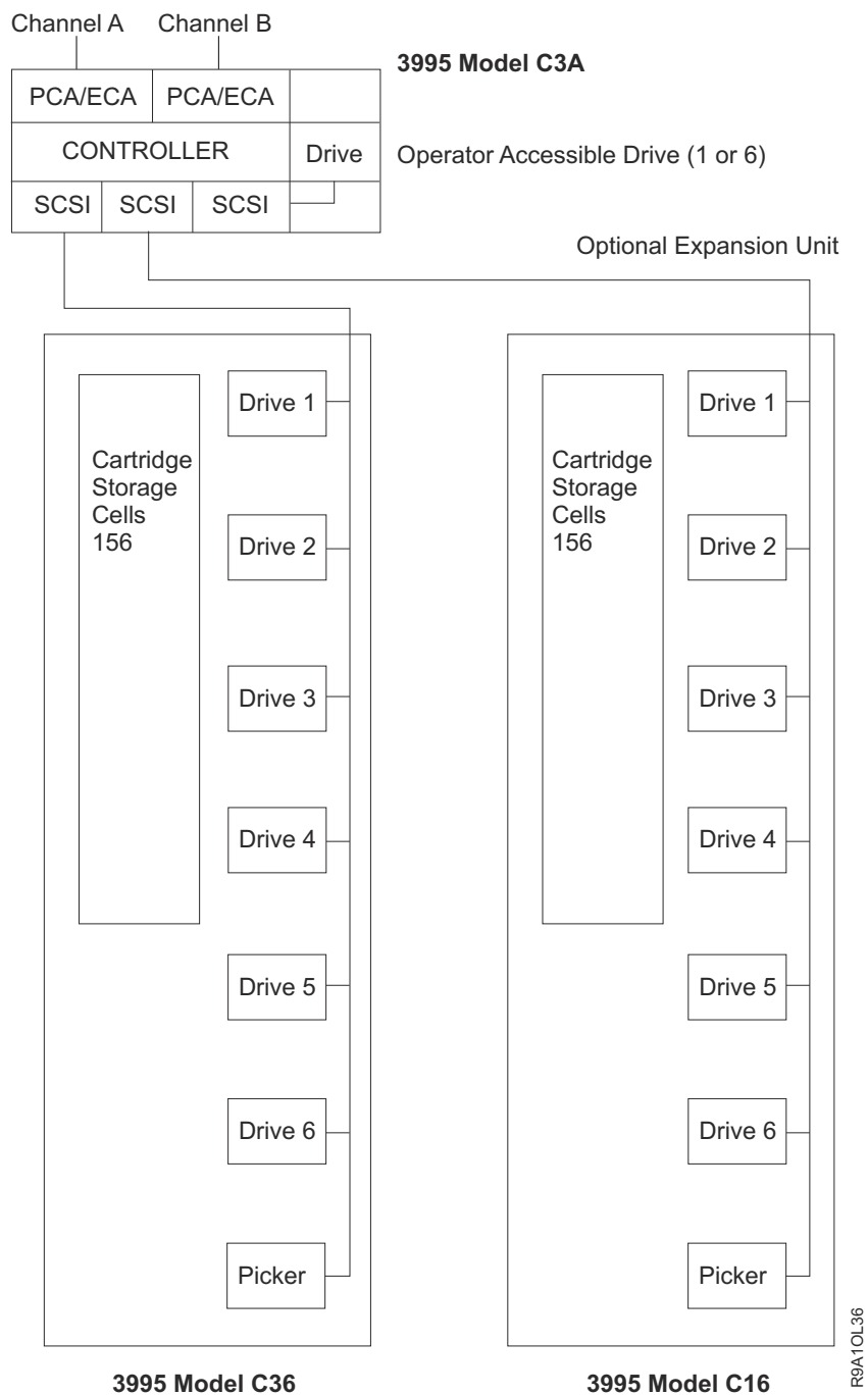
Figure 36. Sample hardware configuration—IBM 3995 model C3A, C36, and C16
