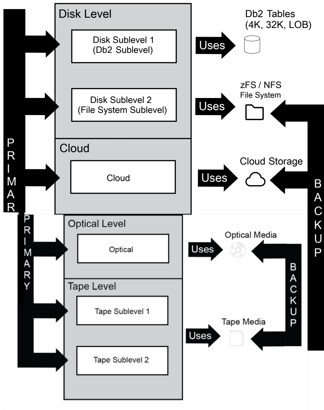
Figure 1. Object storage hierarchy
