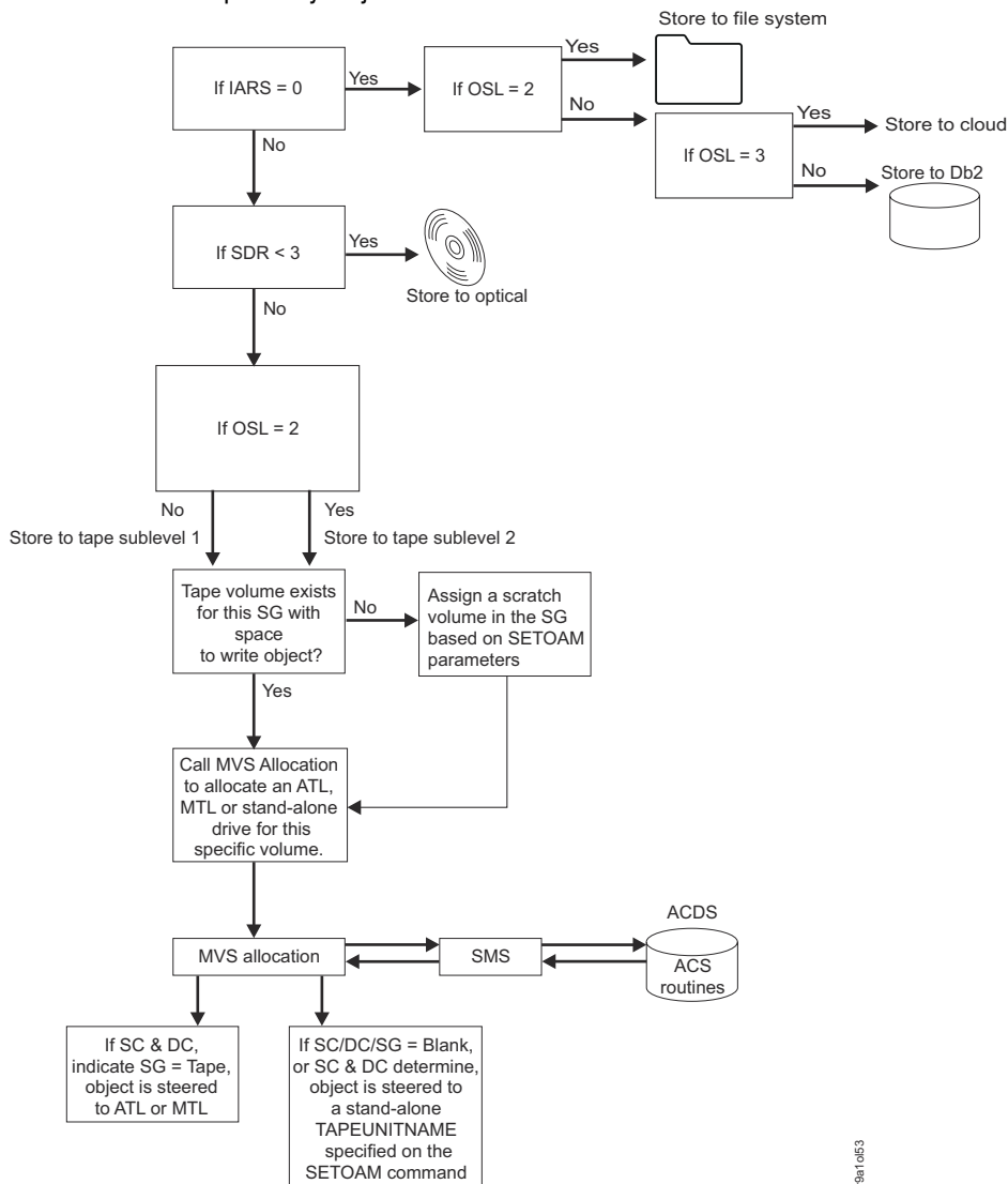
Figure 5. Conceptual overview of storing a primary object
